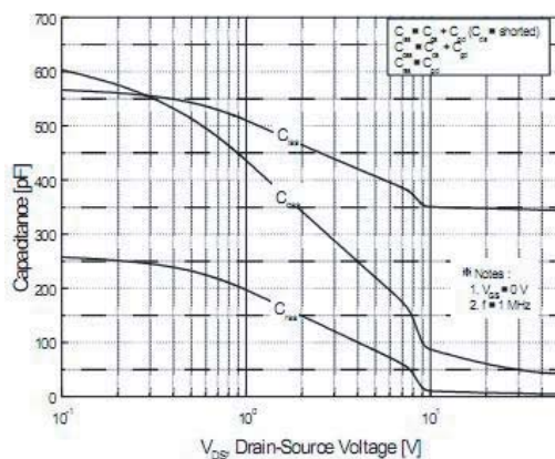
Figure 5. Capacitance Characteristics
