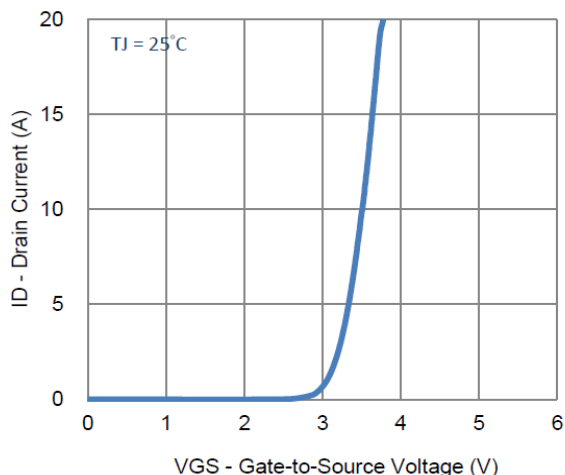
2. Transfer Characteristics
