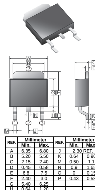
TO-252(D-Pack)
