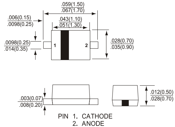
SOD-523
