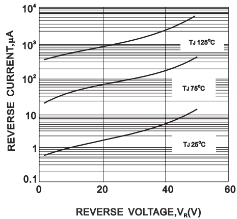
FIG. 2-TYPICAL REVERSE CHARACTERISTIC
