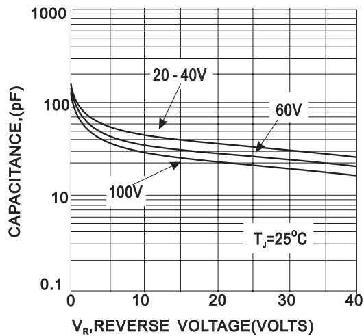
FIG. 3-TYPICAL JUNCTION CHARACTERISTIC
