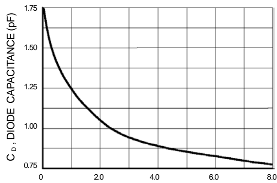
Figure 4. Capacitance
