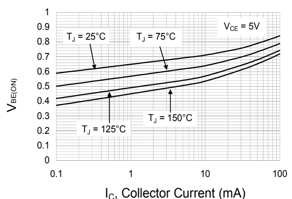
Fig.4 Base-Emitter Voltage vs. Collector Current
