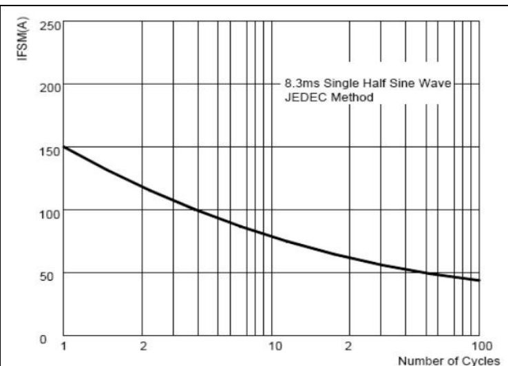
FIG.2-MAXFWD NON-REPETITIVE FORWARD SUGE CURRENT
