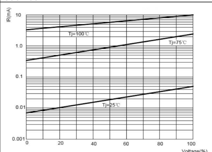
FIG.4-TYPICAL REVERSE CHARACTERISTIC
