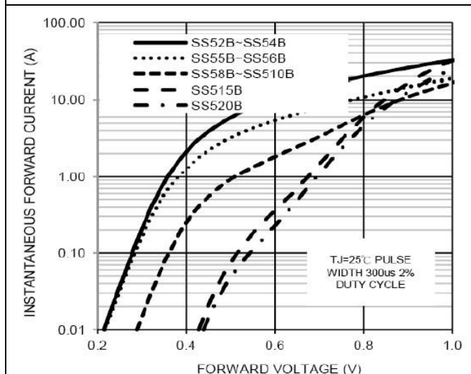
FIG.3-TYPICAL FORWARD CHARACTERISTICS
