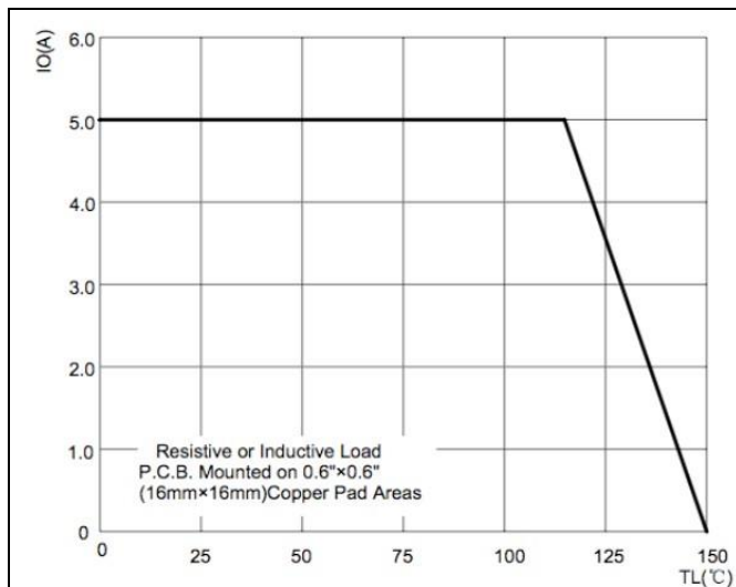
FIG.1-FORWARD DERATIVE CURVE
