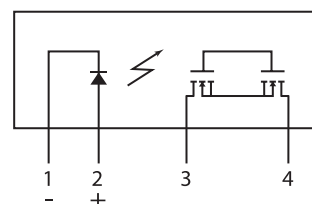
CPC1973Y Pinout
