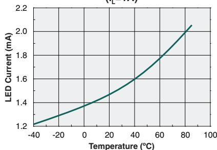
Typical I_F for Switch Operation ( I_L=1\text{A} )
