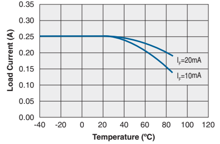
Typical Maximum DC Load Current vs. Temperature
